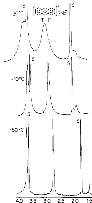
Figure 1. 1 H NMR spectrum of anthracene dianion (5) in THF at various temperatures. S refers to the solvent signals. See ref 27.
